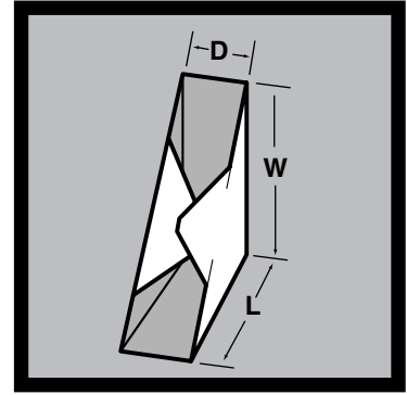
TRIANGULAR PAD
